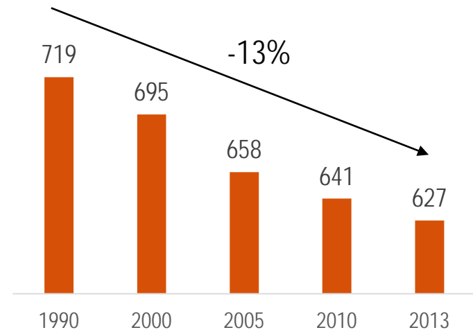
Evolution of CO 2 emissions per ton of cement produced in EU28 (kg CO 2 /ton Grey and white cementitious*)
