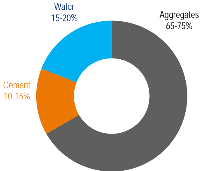
Composition of concrete by volume
